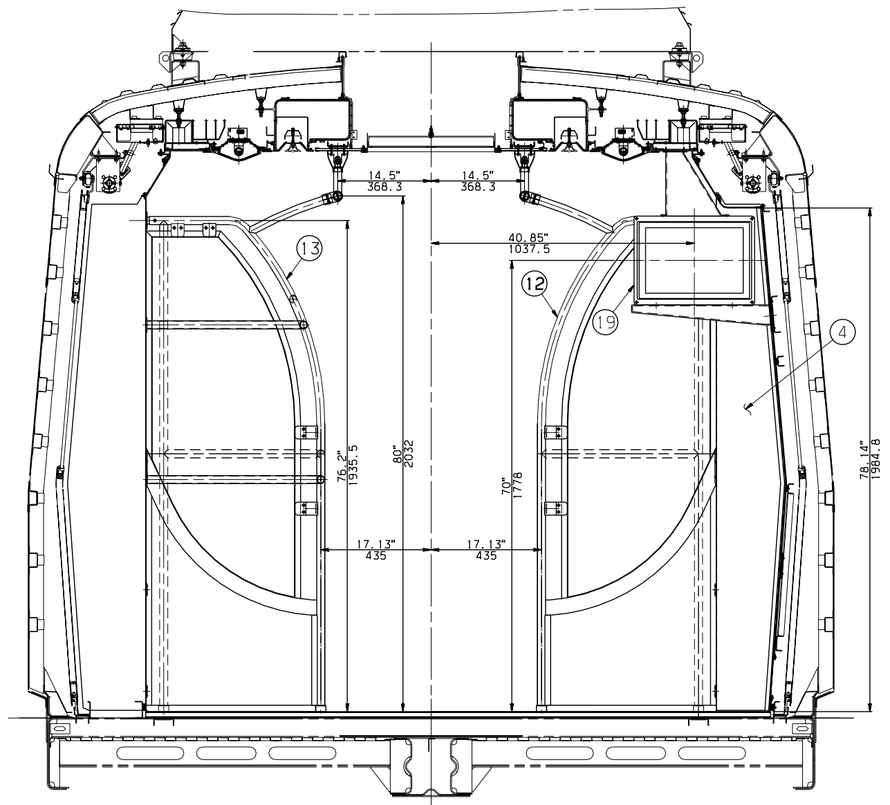
SECTION E-E
